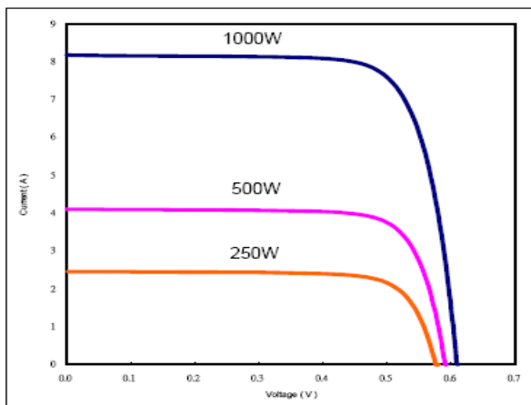
IV - Curve
